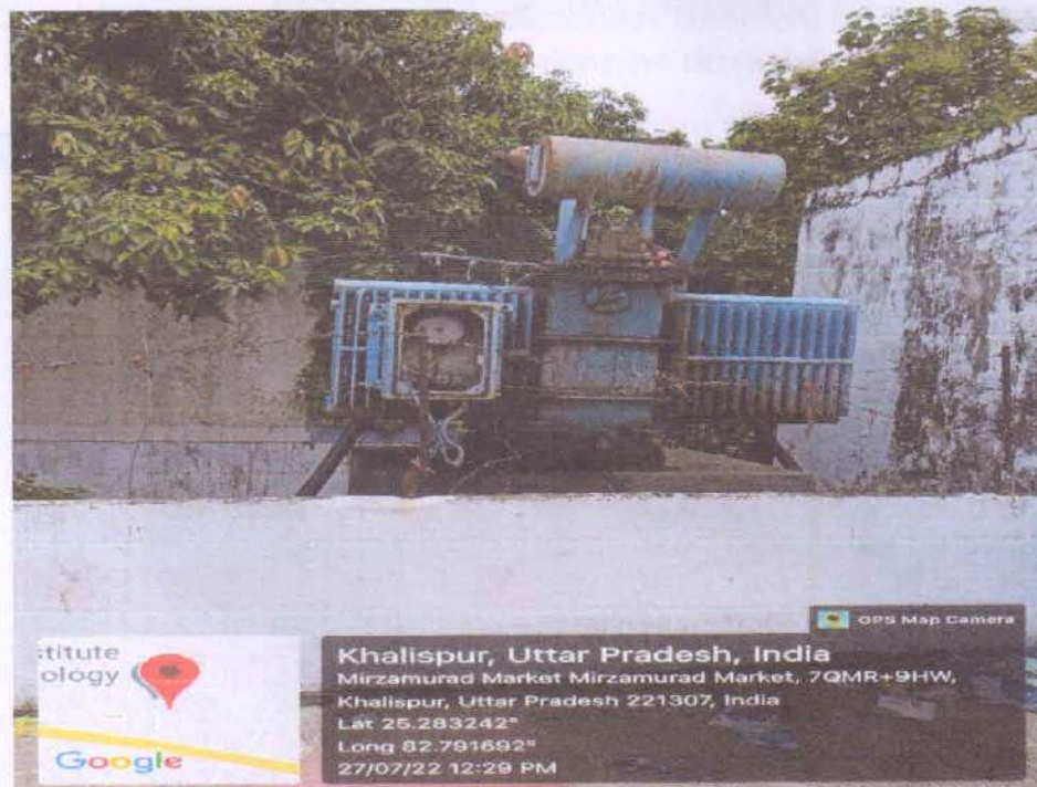
Fig-4.1: 11/0.4 Transformer (650 KVA)
